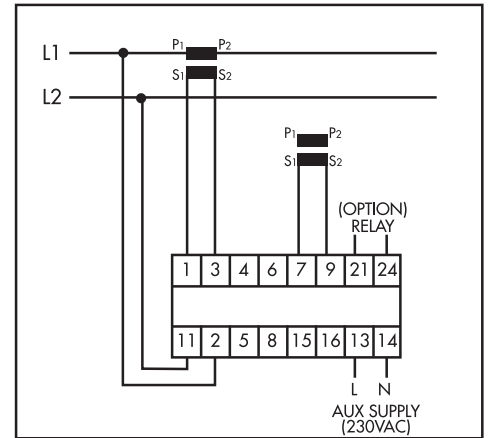
Figure 3 :- Single Phase
