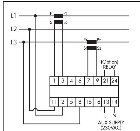
Figure 2 :- 3P3W
